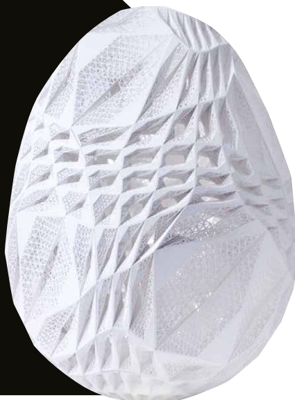
grade architecture
